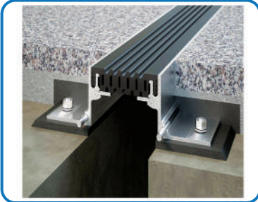
Expansion Joint System
