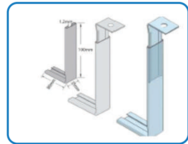
Adjustable Head Restraint IAHR)
