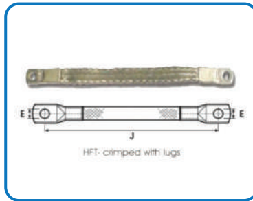
H F T - Crimped with Lugs
