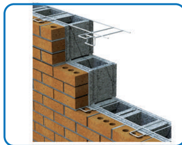
Block Reinforcement (Ladder Type & Truss Type)
